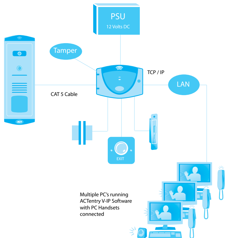
ACTentry V-IP System Schematic
